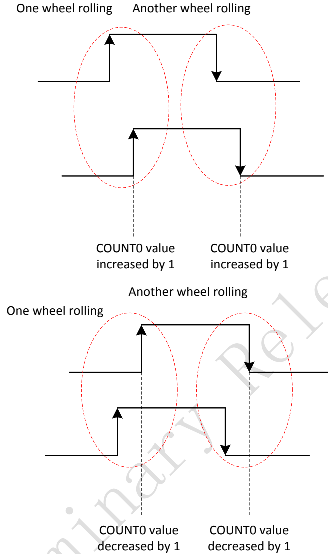
Figure 9- 1 Common mode
