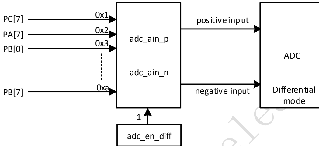
Figure 10- 1 Block diagram of ADC
