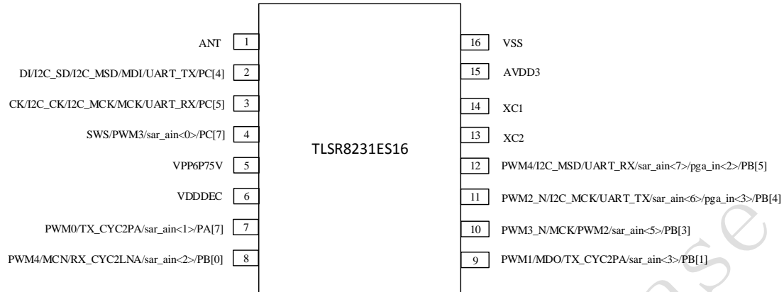
Figure 1- 5 Pin assignment for TLSR8231ES16
