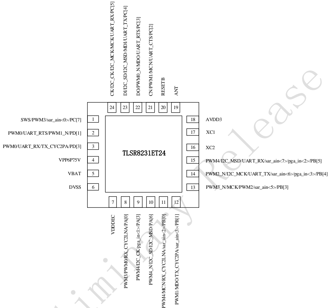
Figure 1- 4 Pin assignment for TLSR8231ET24
