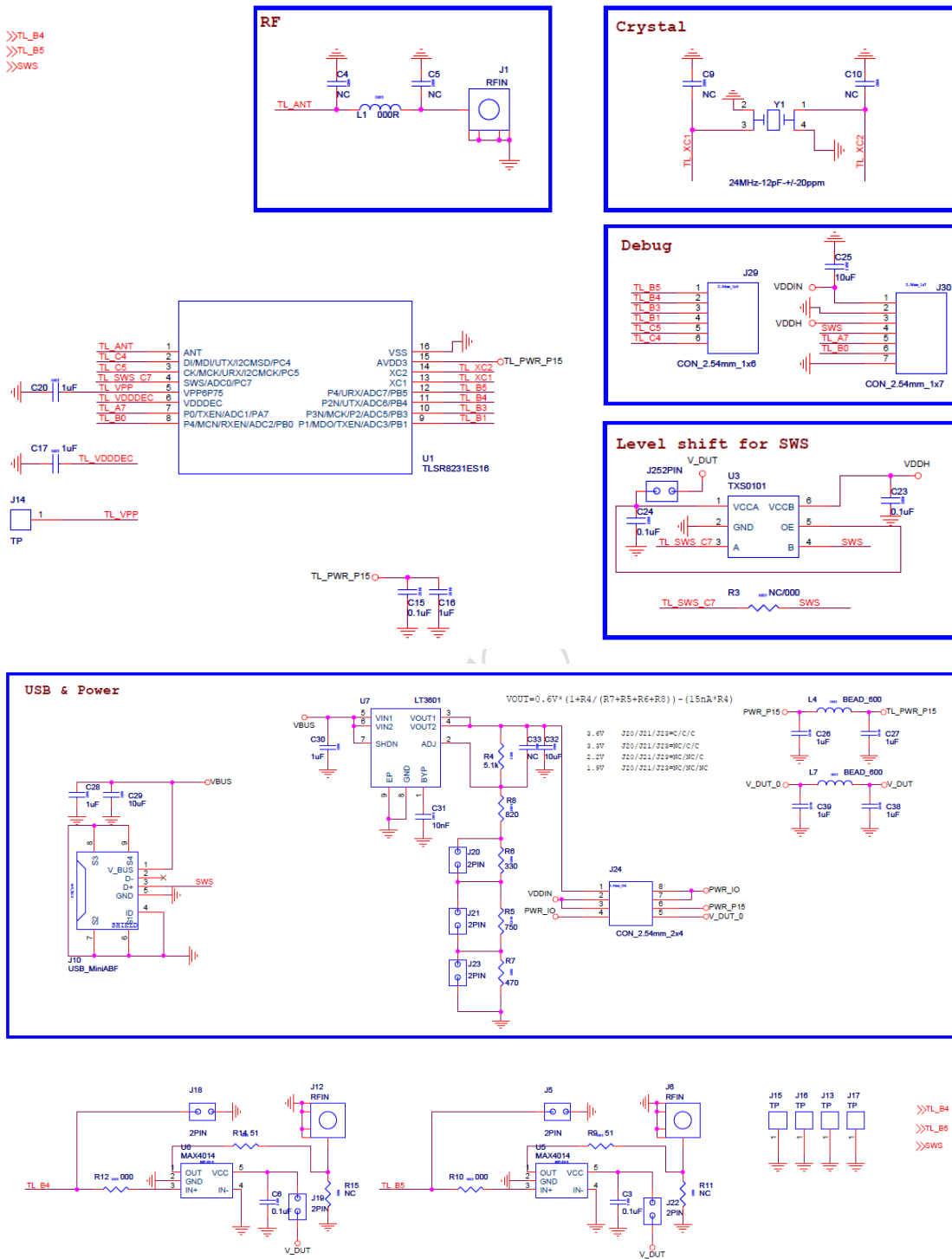
Figure 14- 3 Schematic for TLR8231ES16
