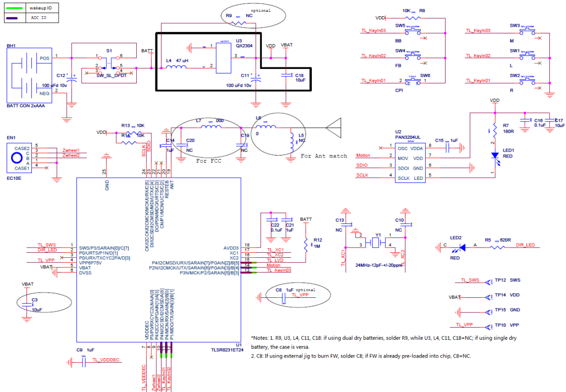
Figure 14- 1 Schematic for TLSR8231ET24
