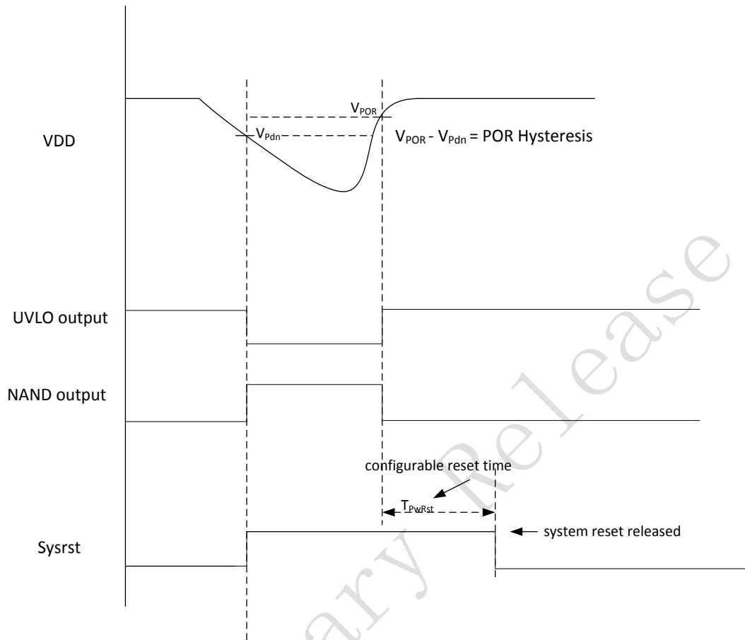
Figure 2- 6 Power-down sequence
